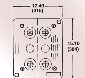
TWO CELL UNIT GT 9 TO 13 PLATE PERPENDICULAR PLATE ORIENTATION
