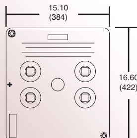
SINGLE CELL UNIT GT 23 TO 45 PLATE PARALLEL PLATE ORIENTATION
