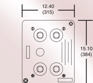
SINGLE CELL UNIT GT 15 TO 21 PLATE PERPENDICULAR PLATE ORIENTATION
