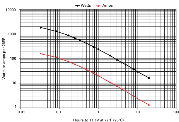
Figure B-12: 26EP discharge data to 11.1V at 77°F (25°C)
