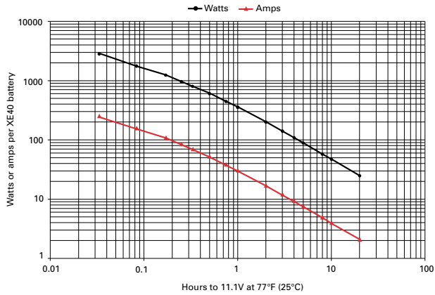
Figure A-16: XE40 discharge data to 11.1V at 77°F (25°C)
