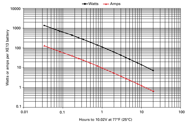
Figure A-2: XE13 discharge data to 10.02V at 77°F (25°C)
